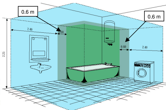
Figure 1: Classification of the Bathroom Zones
